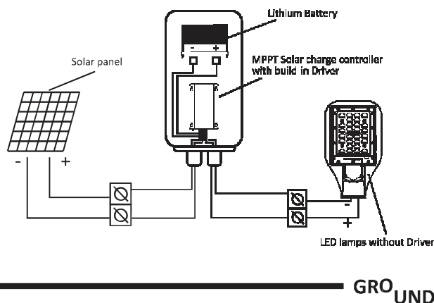
Parts Connection Diagram
